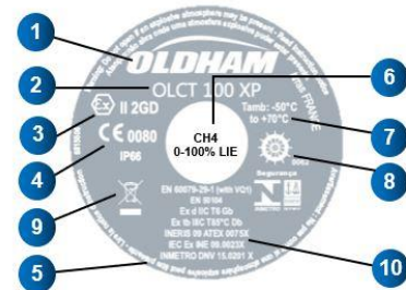
Figure 3 : Firmplate (example)
