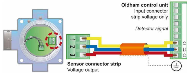
Figure 11: connection for a 3-wire OLC 100 type detector
