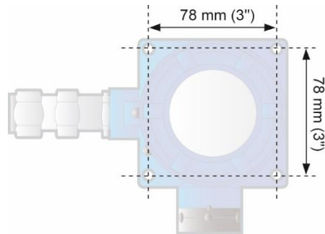
Figure 6 : fixing template for the enclosure
