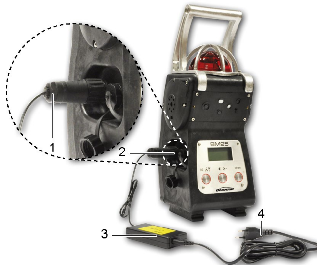
Figure 10: charging in safe area
