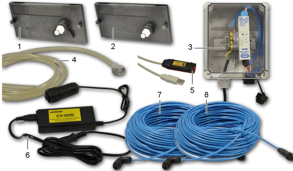
Figure 3: accessories
